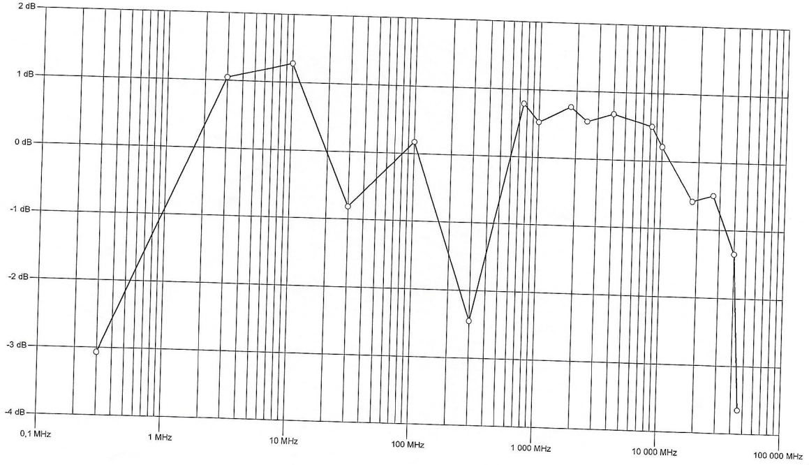
Frequency Response
