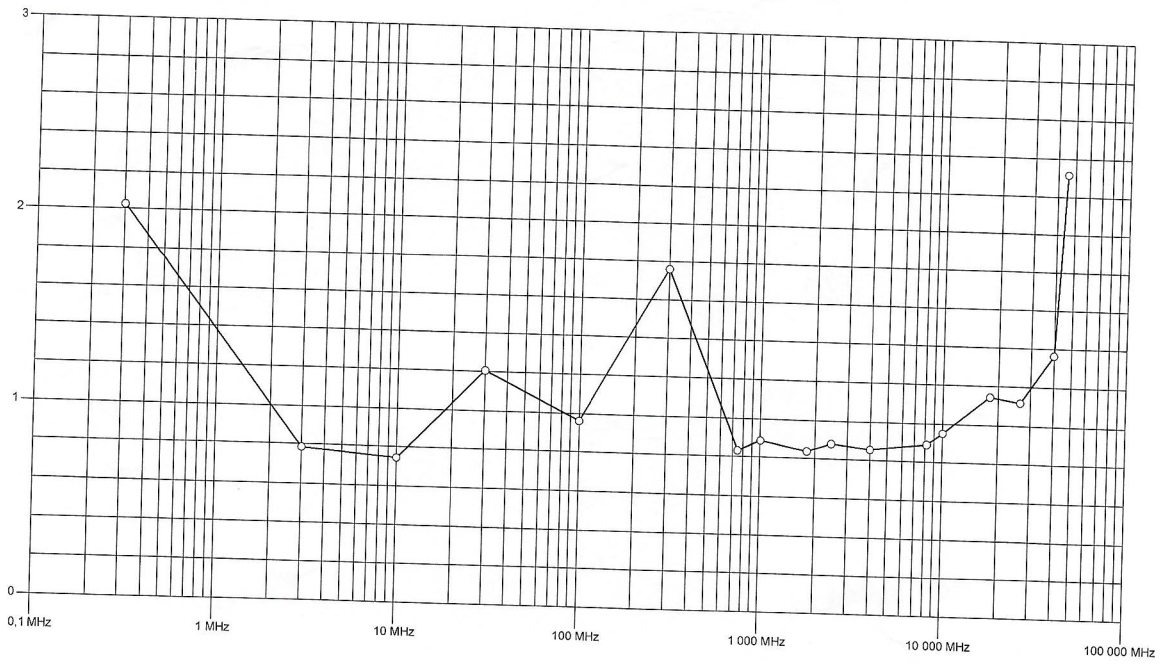
Correction Factor
