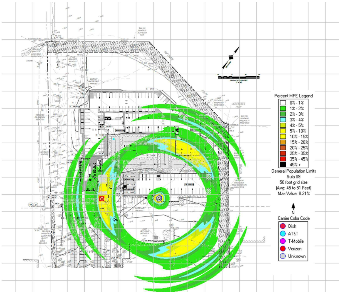
Figure-2 – calculated lower residential roof peak and cupola peak (45') elevation of the premium parking and auto service building cumulative exposure level surrounding the existing telecommunications facility expressed in percentage of the general public FCC standard.
