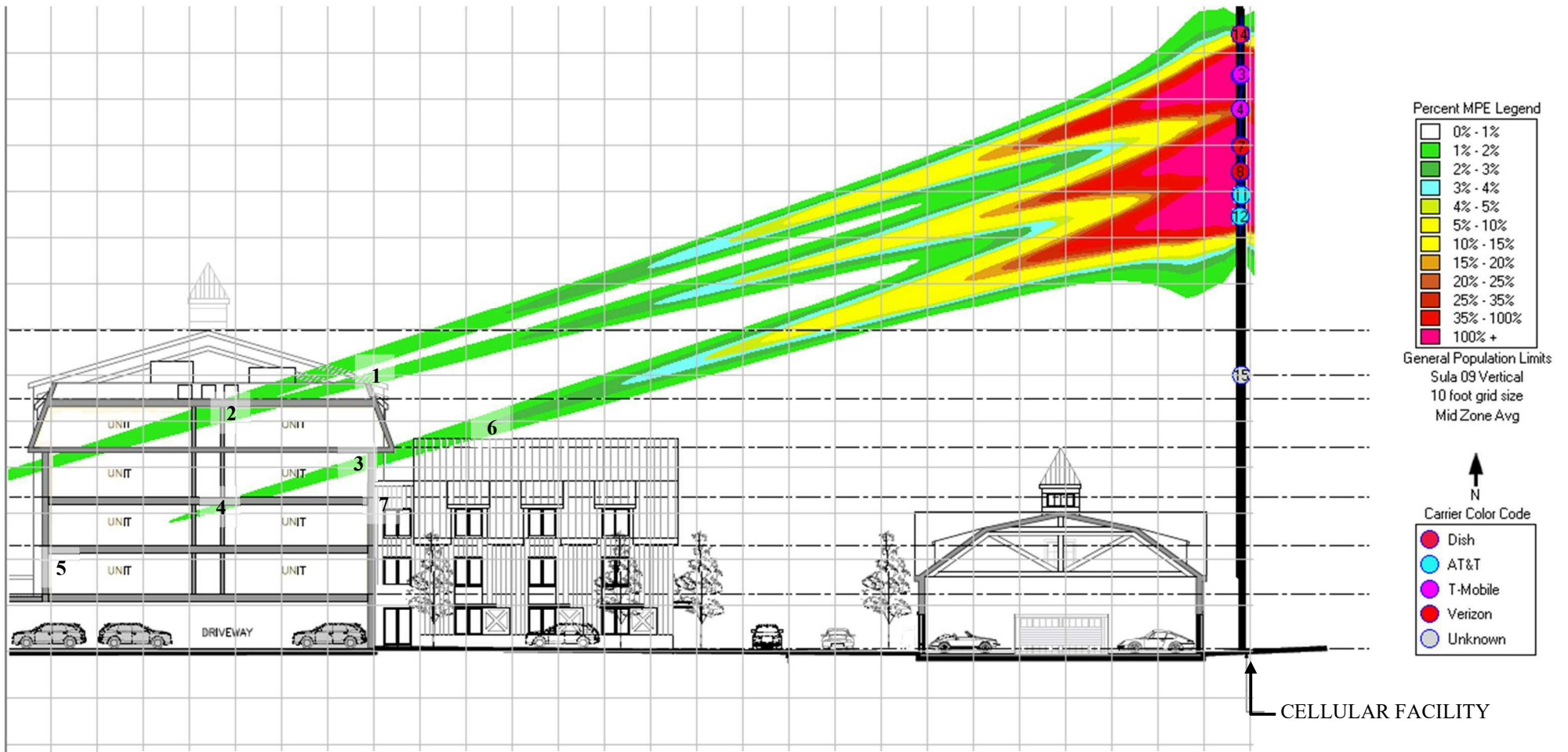
Figure-8 – calculated elevation view exposure level in the 1900 MHz band surrounding the existing telecommunications facility expressed in percentage of the general public FCC standard. Only the significantly elevated pink shaded areas would exceed the general public FCC standard.
