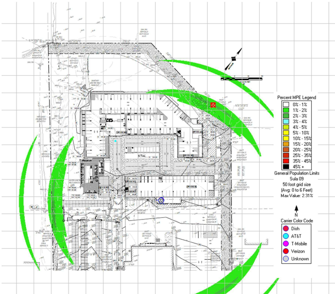
Figure-1 – calculated ground level cumulative exposure level surrounding the existing telecommunications facility expressed in percentage of the general public FCC standard.
