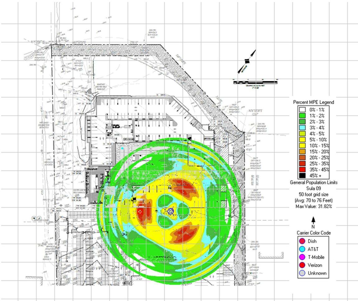
Figure-3 – calculated main rooftop peak (70') of multi-family residential building elevation cumulative exposure level surrounding the existing telecommunications facility expressed in percentage of the general public FCC standard.
