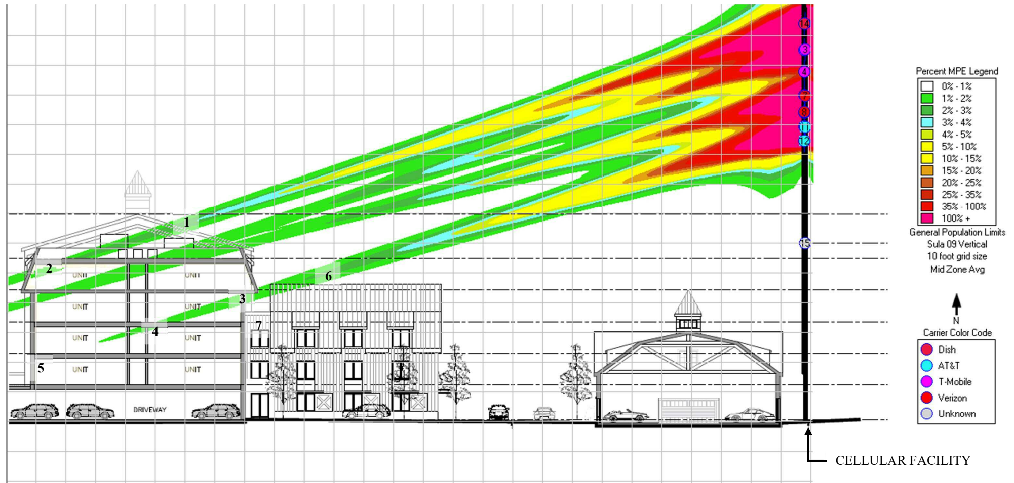
Figure-9 – calculated elevation view exposure level in the 2100 MHz band surrounding the existing telecommunications facility expressed in percentage of the general public FCC standard. Only the significantly elevated pink shaded areas would exceed the general public FCC standard.
