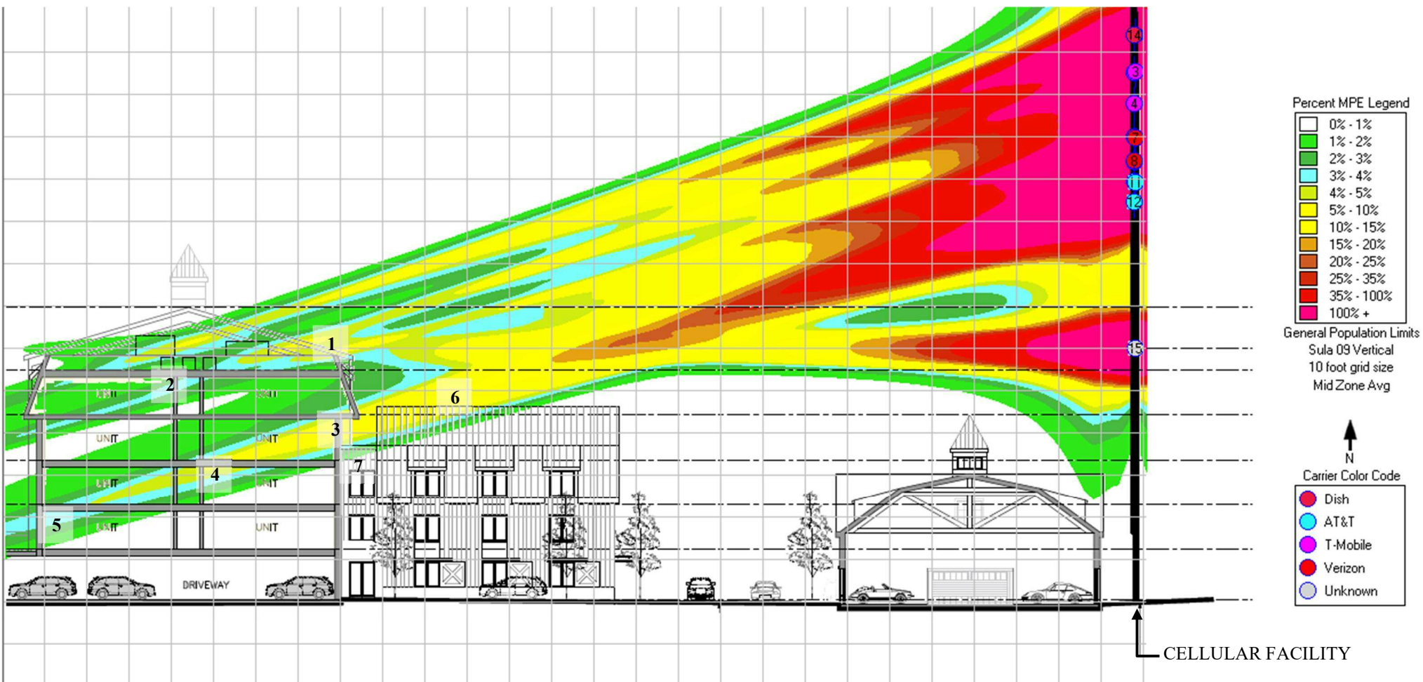
Figure-10 – cumulative calculated elevation view exposure level surrounding the existing telecommunications facility expressed in percentage of the general public FCC standard. Only the significantly elevated pink shaded areas would exceed the general public FCC standard.
