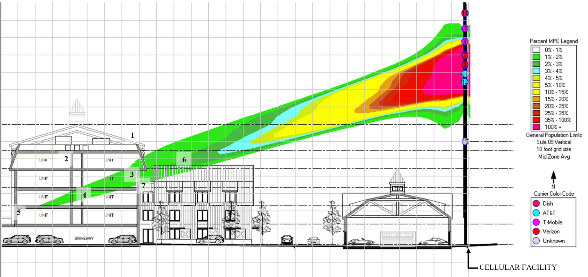
Figure-7 – calculated elevation view exposure level in the 850 MHz band surrounding the existing telecommunications facility expressed in percentage of the general public FCC standard. Only the significantly elevated pink shaded areas would exceed the general public FCC standard.
