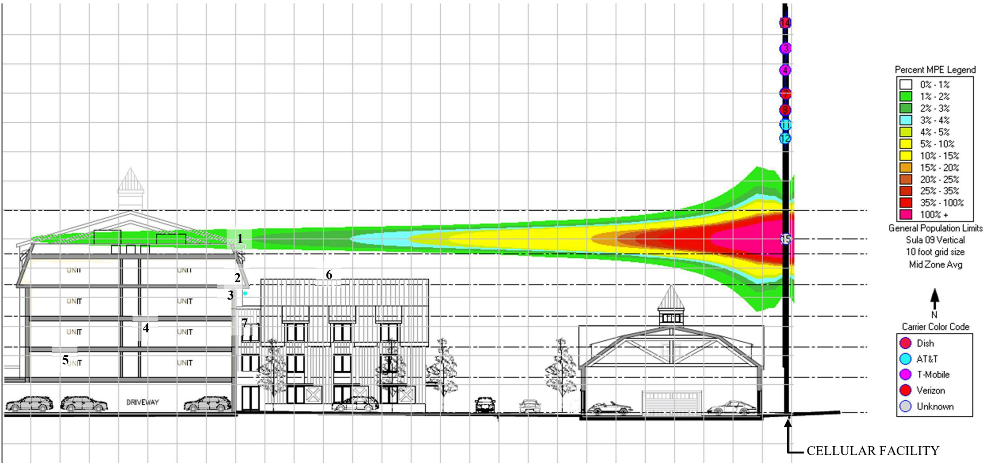
Figure-4 –calculated elevation view exposure level in the 450 MHz band surrounding the existing telecommunications facility expressed in percentage of the general public FCC standard. Only the significantly elevated pink shaded areas would exceed the general public FCC standard.
