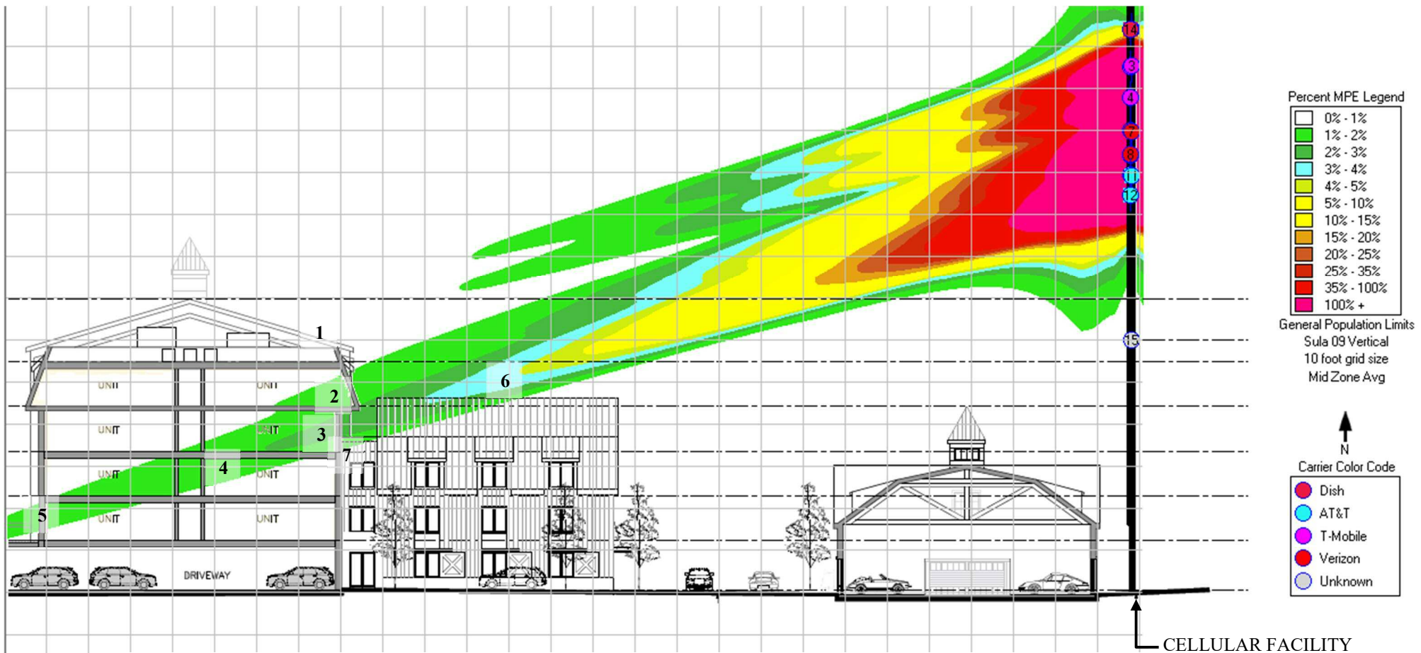
Figure-6 – calculated elevation view exposure level in the 700 MHz band surrounding the existing telecommunications facility expressed in percentage of the general public FCC standard. Only the significantly elevated pink shaded areas would exceed the general public FCC standard.
